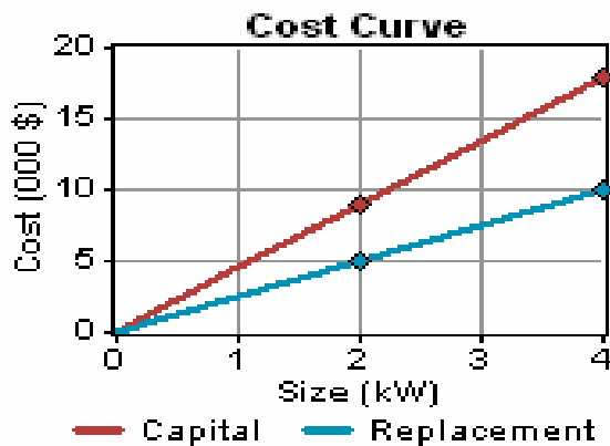
Figure 5. Cost curve of PV
