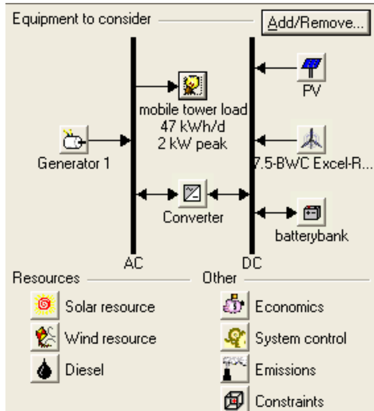
Figure 1. Hybrid system schematic diagram for mobile telephony base station
