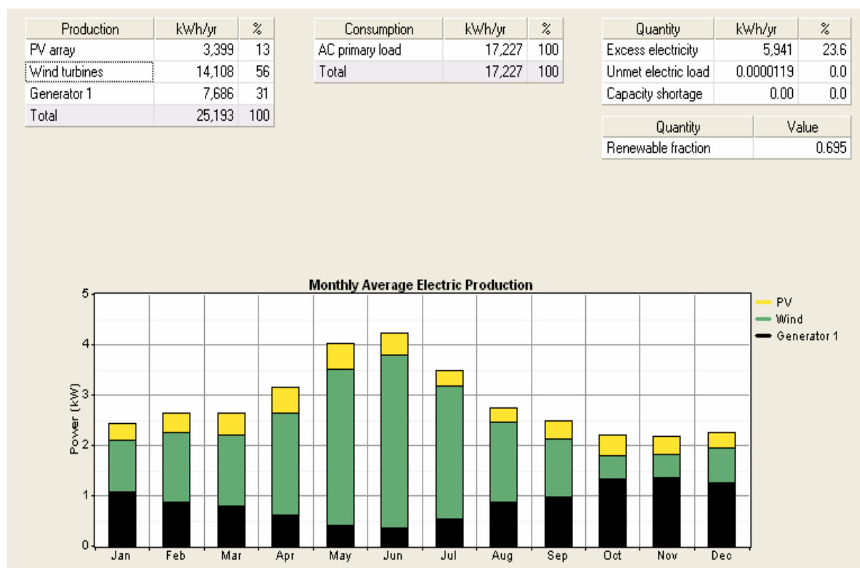
Figure10. Annual electricity production by different hybrid system
