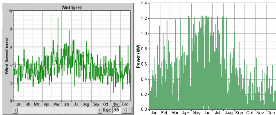
Figure 3. (i) Average hourly wind speed for 1 year, and (ii) wind power output throughout the year
