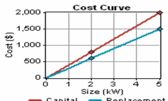
Figure 8. Cost curve of diesel generator
