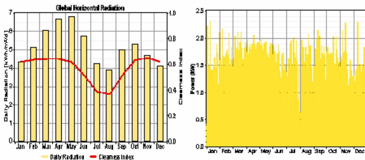
Figure 2. (i) Average daily radiation in a year, and (ii) PV-Power available throughout the year
